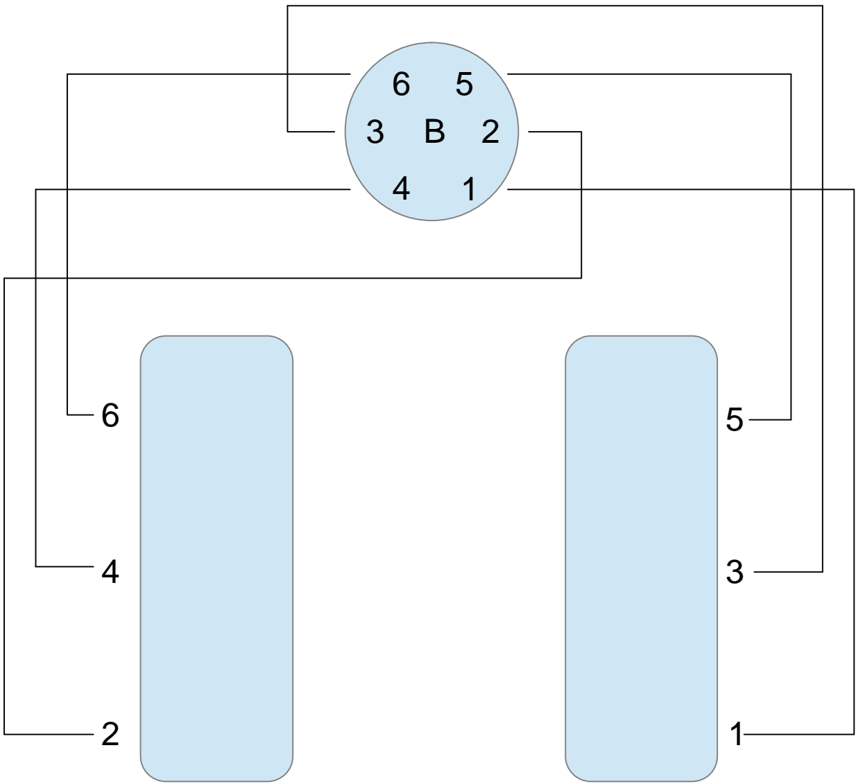
Aurelia Flaminia electronic distributor connection
